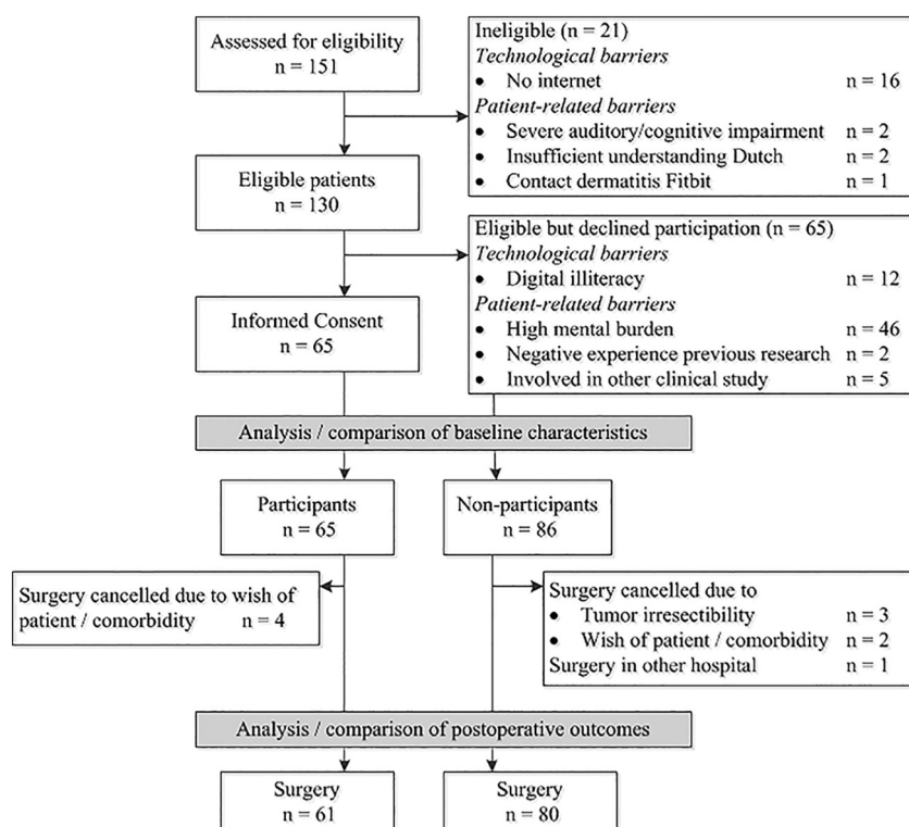
Fig. 1. Study flowchart.
